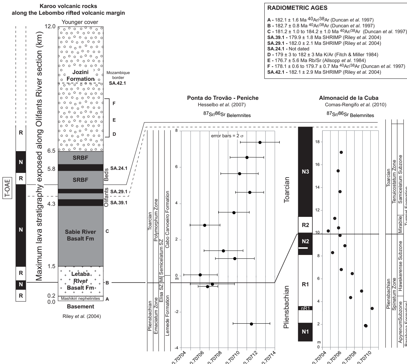
Figure 13. Proposed correlations between Peniche ages and strontium isotope curve with magnetostratigraphy of the Almonacid de la Cuba section and the Karoo volcanic rocks in South Africa. Mi = Mirabile Subzone.
